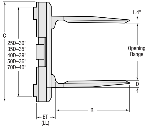
40D Standard Ribbs
